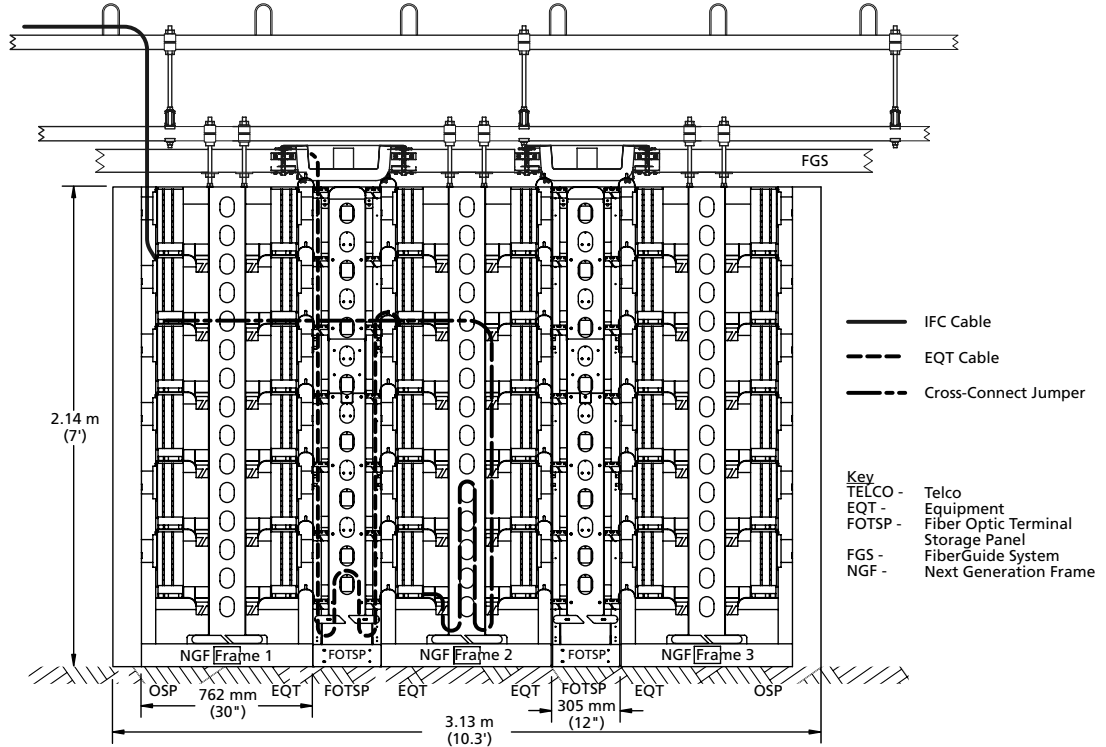
Cross-Connect Application using 12-inch wide FOTSP in a 2:1 Application (2 Equipment to 1 OSP)
