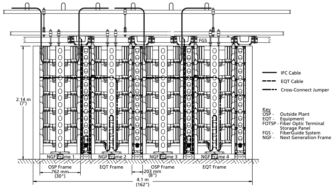
Cross-Connect Application using 8-inch wide FOTSP in a 1:1 Application (1 Equipment to 1 OSP)
