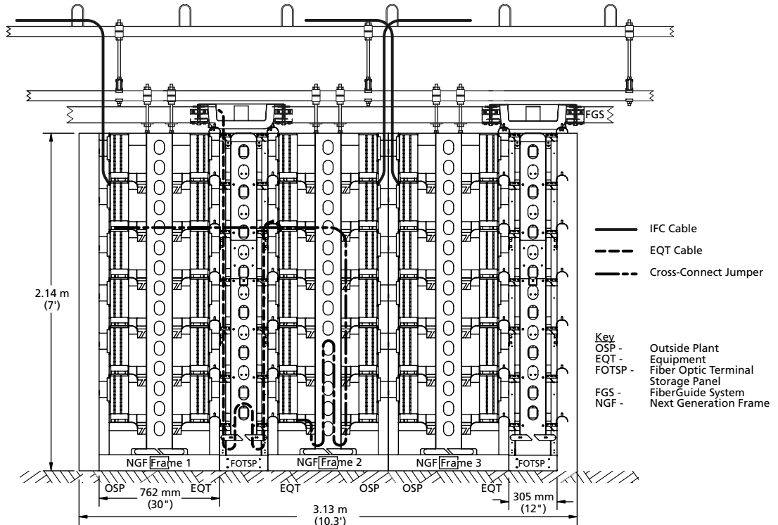
Cross-Connect Application using 12-inch wide FOTSP in a 1:1 Application (1 Equipment to 1 OSP)
