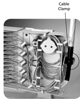
72-Position FTB Loaded with Multifiber Breakout Cable
