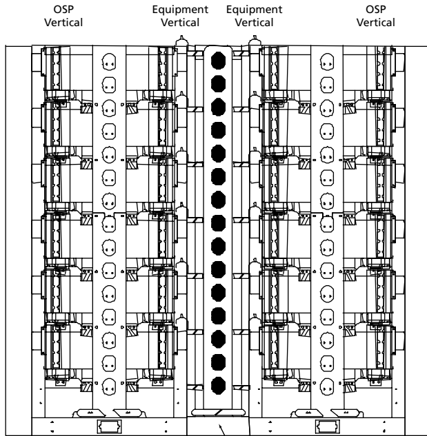
Zoned by Vertical
